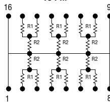
V.35 Termination Network 16 Pin
